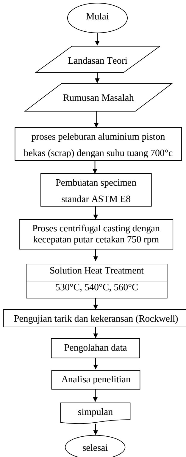
Gambar 34. diagram alir
